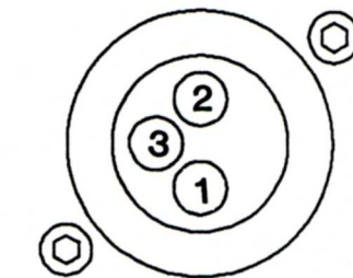
XLR PINOUT (INPUTS-FEMALE)
